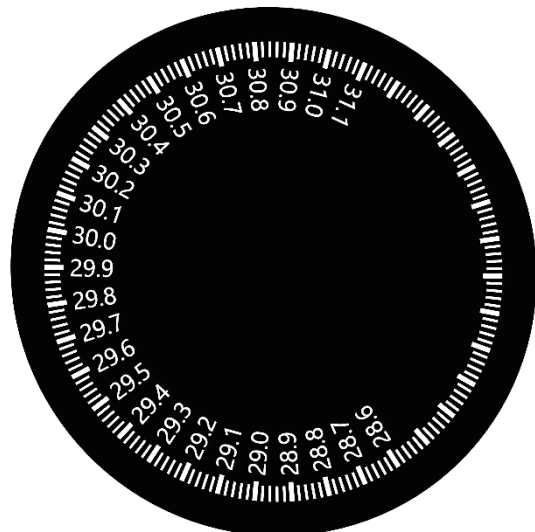
Baro Scale (Diameter 69mm)
